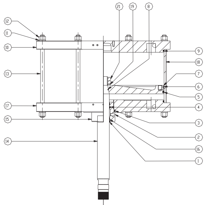
PNEUMATIC PISTON CYLINDER
