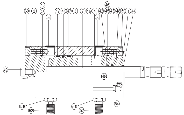
HYDRAULIC CYLINDER
