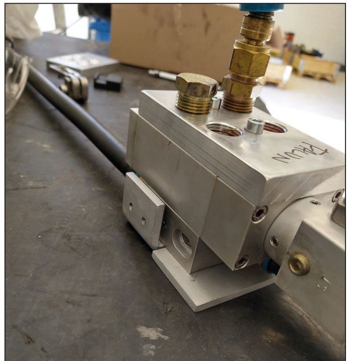
MOUNTING BRACKET FOR PILOT VALVE
